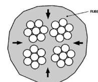
Open steel cords SIDERFLEX IW-HE
